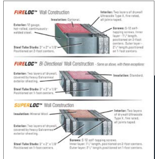
Fire-rated wall construction with tubular supports.
