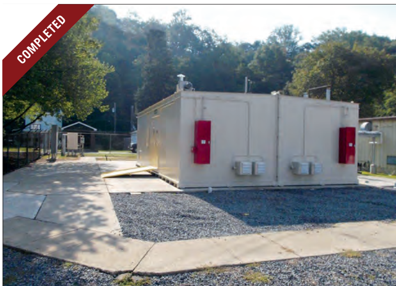
Modular chemical storage building with double leaf doors, mechanical ventilation, and integral dry chemical fire suppression systems.
