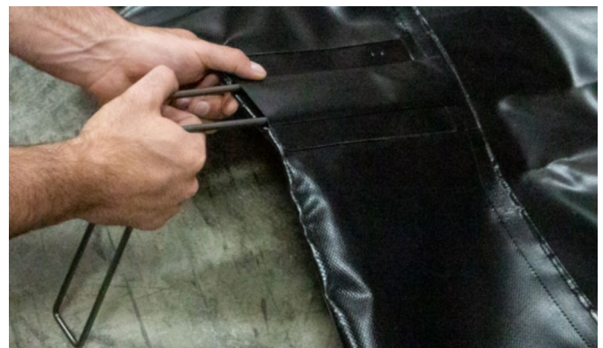
Slip angle L-brackets into protective pockets to keep walls upright, no sagging.
